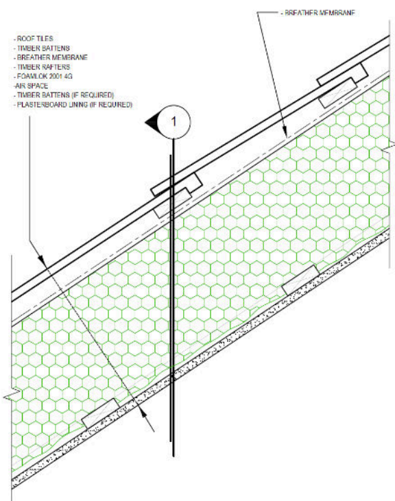
Diagram 1 - Elevation detail of typical loft application (at roof line)
