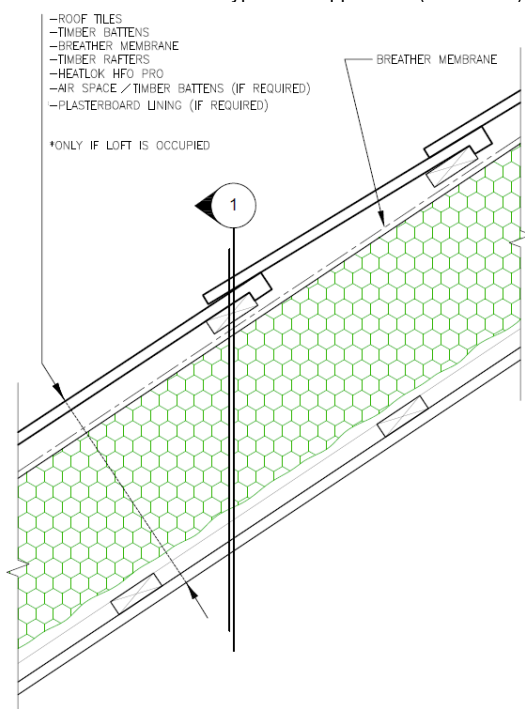
Diagram 1 - Elevation detail of typical loft application (at roof line)
