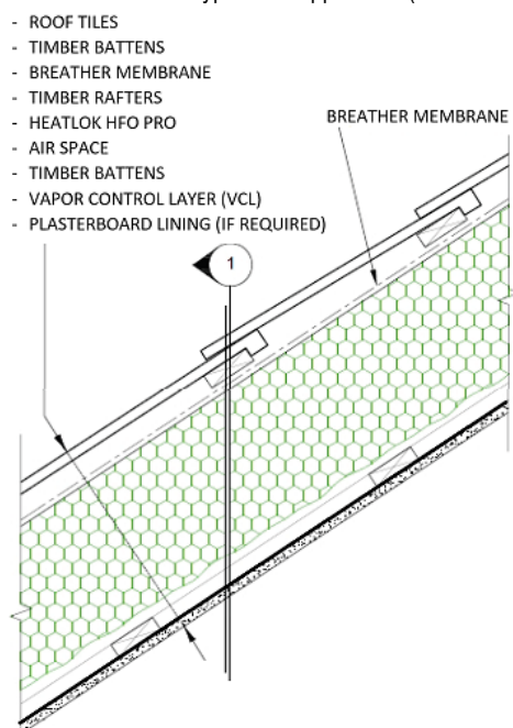
Diagram 1 - Elevation detail of typical loft application (at roof line)
