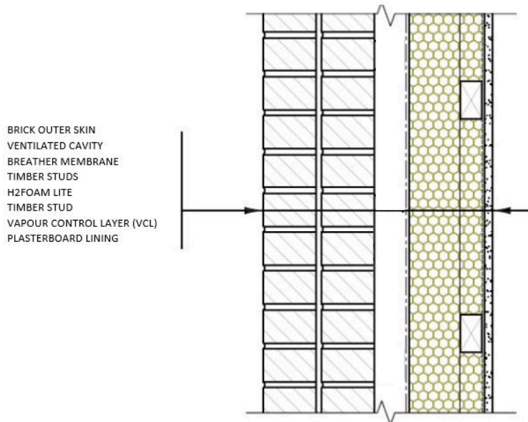
Diagram 1 - Typical detail timber-framed walls with brick outer skin
