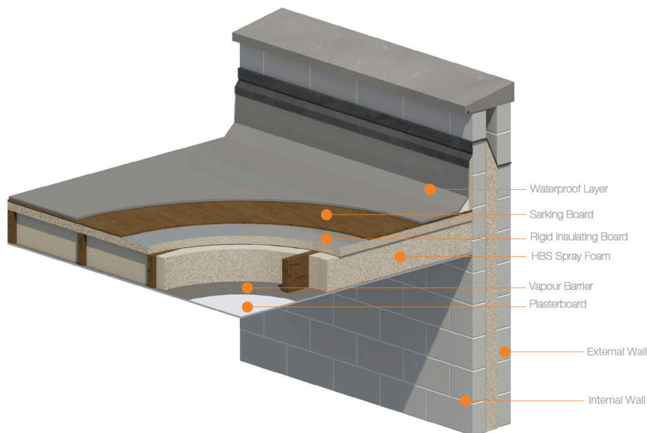
Diagram 1 - detail of typical timber-frame flat roof
