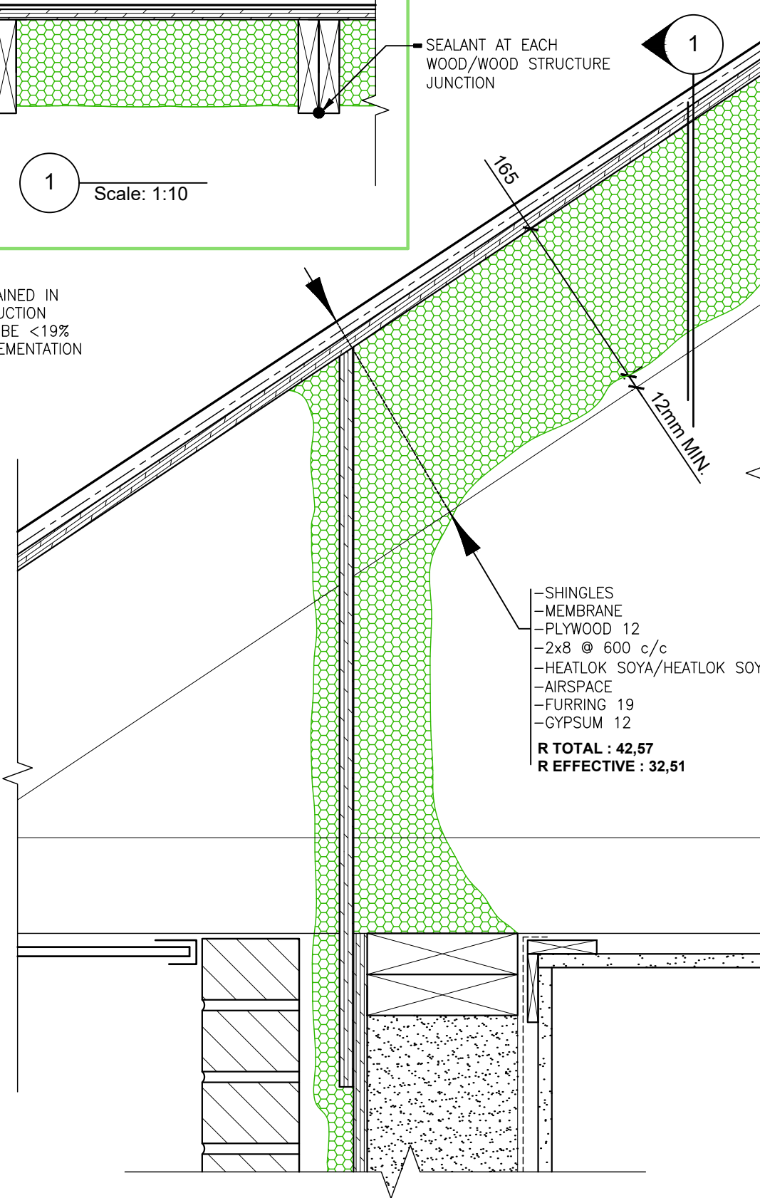
TYPICAL DETAIL - WOOD FRAMING
